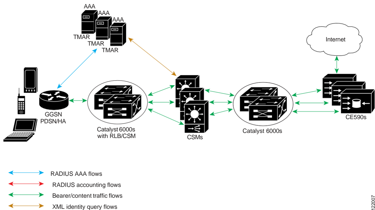
Figure 7-1 Tech Mahindra Access Registrar System Overview
